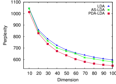
(b) Changed Perplexity on AmazonFood.
