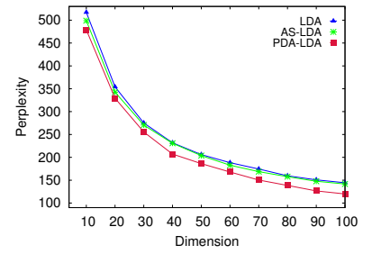
(c) Changed Perplexity on AmazonSport.
