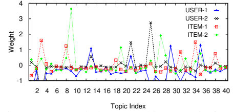
Figure 3: Sampled user and item topic factors.
