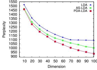
(a) Changed Perplexity on Yelp.
